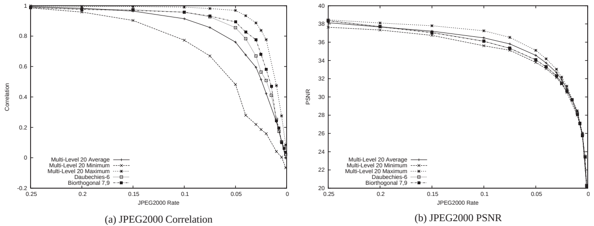
Fig. 17. Correlation and PSNR of multi-level system under JPEG2000 compression: (a) JPEG2000 Correlation, and (b) JPEG2000 PSNR.
