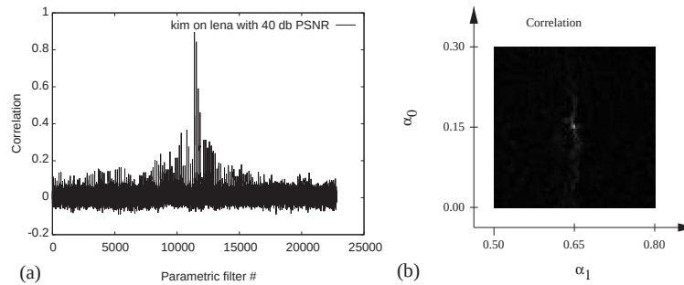
Fig. 4. Kim algorithm: \alpha_0 \in \{0.000, \dots, 0.300\} and \alpha_1 \in \{0.500, \dots, 0.800\} with \Delta = 0.002 .
