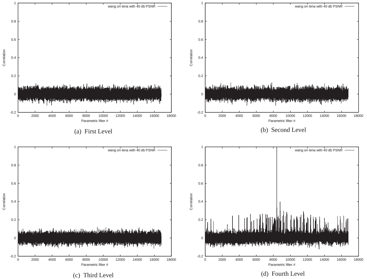
Fig. 14. Attacks on all four levels: (a) first level, (b) second level, (c) third level, and (d) fourth level.
