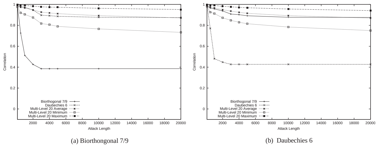
Fig. 21. Fixed quantization of coefficients: details of Multi-Level 20 system: (a) Biorthogonal 7/9, and (b) Daubechies 6.
