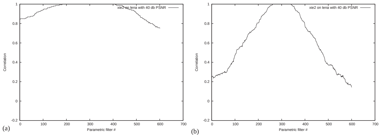
Fig. 9. Xie's algorithm: Variation of only one parameter. Both diagrams use \Delta = 0.0005 . (a) \alpha_1 = 0.650 and \alpha_0 \in \{0.000, \dots, 0.300\} . (b) \alpha_0 = 0.150 and \alpha_1 \in \{0.500, \dots, 0.800\} .
