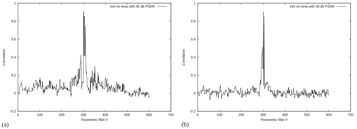
Fig. 5. Kim algorithm: Variation of only one parameter. Both diagrams use \Delta = 0.0005 . (a) \alpha_1 = 0.650 and \alpha_0 \in \{0.000, \dots, 0.300\} . (b) \alpha_0 = 0.150 and \alpha_1 \in \{0.500, \dots, 0.800\} .
