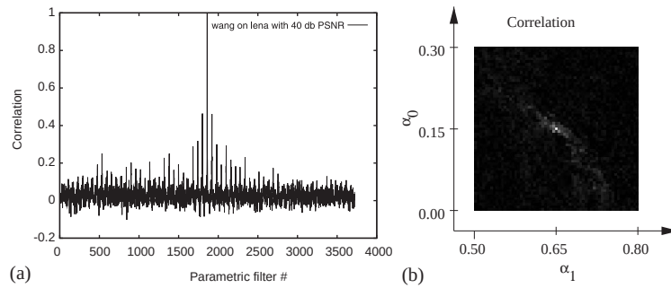
Fig. 6. Wang algorithm: \alpha_0 \in \{0.000, \dots, 0.300\} and \alpha_1 \in \{0.500, \dots, 0.800\} with \Delta = 0.005 .
