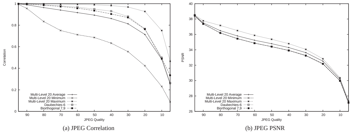
Fig. 18. Correlation and PSNR of multi-level system under JPEG compression: (a) JPEG Correlation, and (b) JPEG PSNR.
