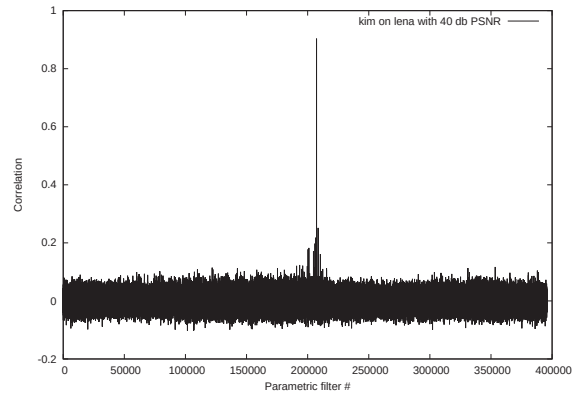
Fig. 3. Kim algorithm. \alpha_0, \alpha_1 \in \{-3.14, -3.13, \dots, 3.13, 3.14\} with \Delta = 0.01 .
