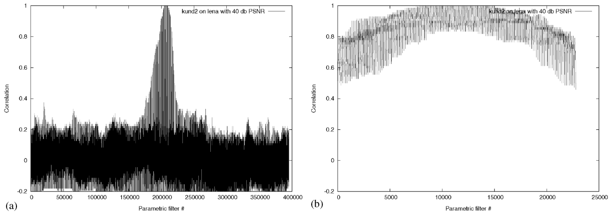
Fig. 7. Kundur algorithm: The watermark was embedded with a PSNR of 40 dB at \alpha_0 = 0.150 and \alpha_1 = 0.650 . (a) \alpha_0, \alpha_1 \in \{-3.14, -3.13, \dots, 3.13, 3.14\} with \Delta = 0.01 . (b) \alpha_0 \in \{0.000, \dots, 0.300\} and \alpha_1 \in \{0.500, \dots, 0.800\} with \Delta = 0.002 .
