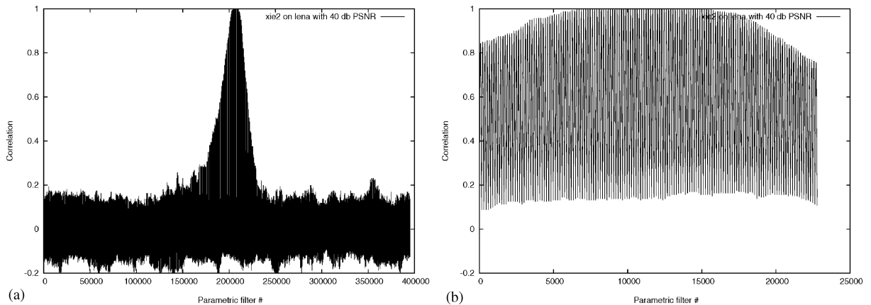
Fig. 8. Xie algorithm: The watermark was embedded with a PSNR of 40 dB at \alpha_0 = 0.150 and \alpha_1 = 0.650 . (a) \alpha_0, \alpha_1 \in \{-3.14, -3.13, \dots, 3.13, 3.14\} with \Delta = 0.01 . (b) \alpha_0 \in \{0.000, \dots, 0.300\} and \alpha_1 \in \{0.500, \dots, 0.800\} with \Delta = 0.002 .
