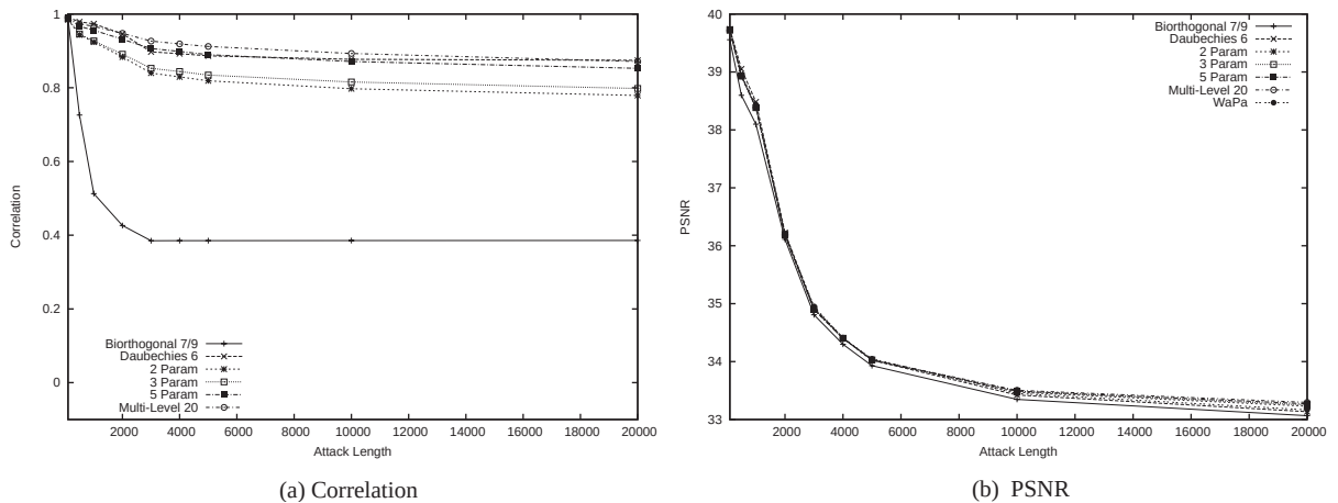
Fig. 19. Fixed quantization of coefficients after Biorthogonal 7/9 decomposition: (a) Correlation, and (b) PSNR.
