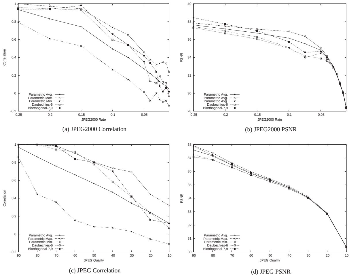
Fig. 12. Correlation and PSNR of Kundur's watermarking algorithm under JPEG and JPEG2000 compression: (a) JPEG2000 Correlation, (b) JPEG2000 PSNR, (c) JPEG Correlation, and (d) JPEG PSNR.
