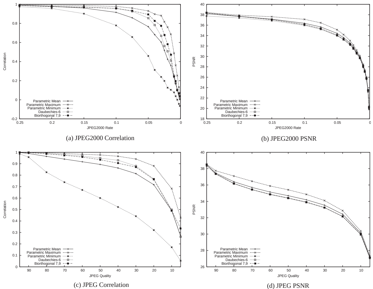
Fig. 11. Correlation and PSNR of Wang watermarks under JPEG and JPEG2000 compression: (a) JPEG2000 Correlation, (b) JPEG2000 PSNR, (c) JPEG Correlation, and (d) JPEG PSNR.
