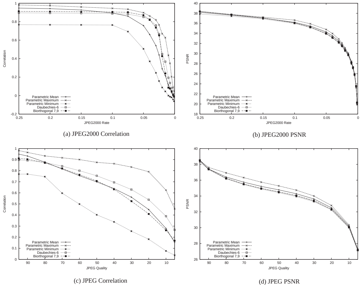
Fig. 10. Correlation and PSNR of Kim watermarks under JPEG and JPEG2000 compression: (a) JPEG2000 Correlation, (b) JPEG2000 PSNR, (c) JPEG Correlation, and (d) JPEG PSNR.
