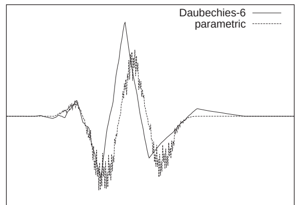
Fig. 2. Comparison of standard Daubechies 6 and a parametrized wavelet filter using \alpha_0 = -0.4815 and \alpha_1 = 2.6585 .
