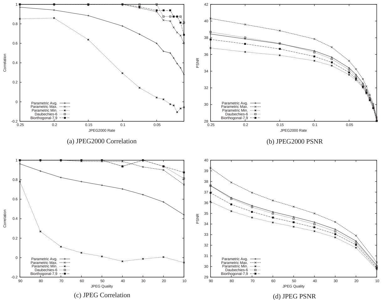
Fig. 13. Correlation and PSNR of Xie's watermarking algorithm under JPEG and JPEG2000 compression: (a) JPEG2000 Correlation, (b) JPEG2000 PSNR, (c) JPEG Correlation, and (d) JPEG PSNR.
