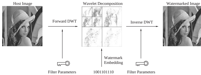
Fig. 1. Overview of watermark embedding procedure using parametrized wavelet filters.
