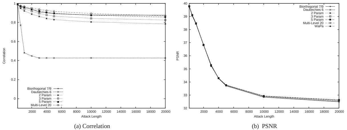
Fig. 20. Fixed quantization of coefficients after Daubechies 6 decomposition: (a) Correlation, and (b) PSNR.
